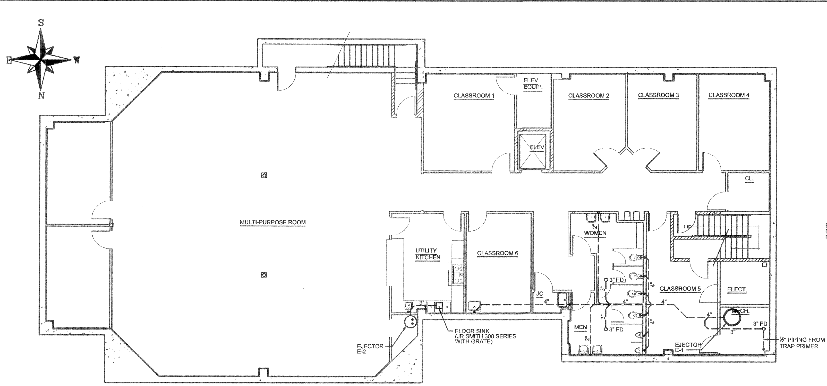
BASEMENT UNDERGROUND PIPING PLAN
