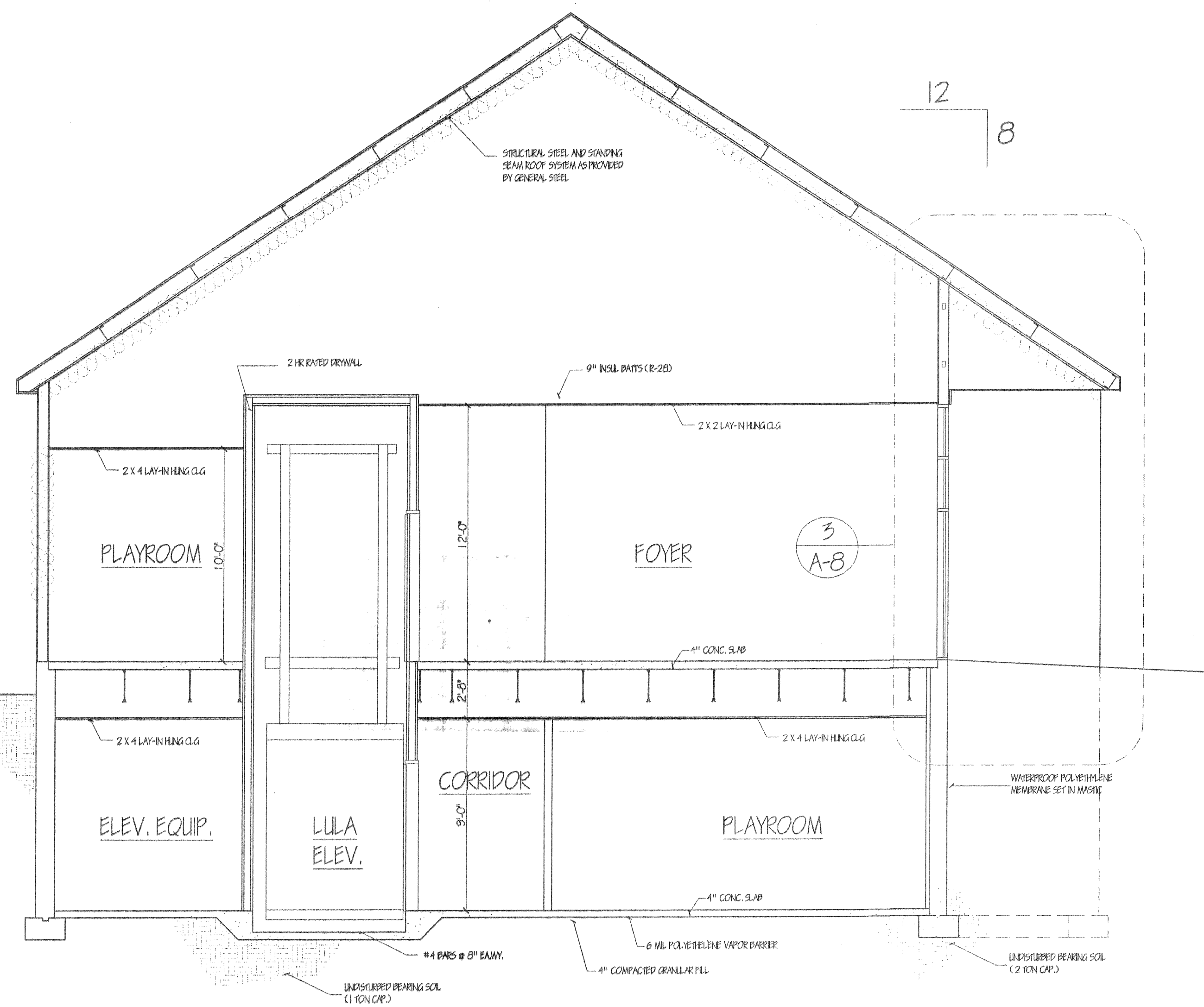
SECTION 1 A-7 1/4" = 1'-0"
