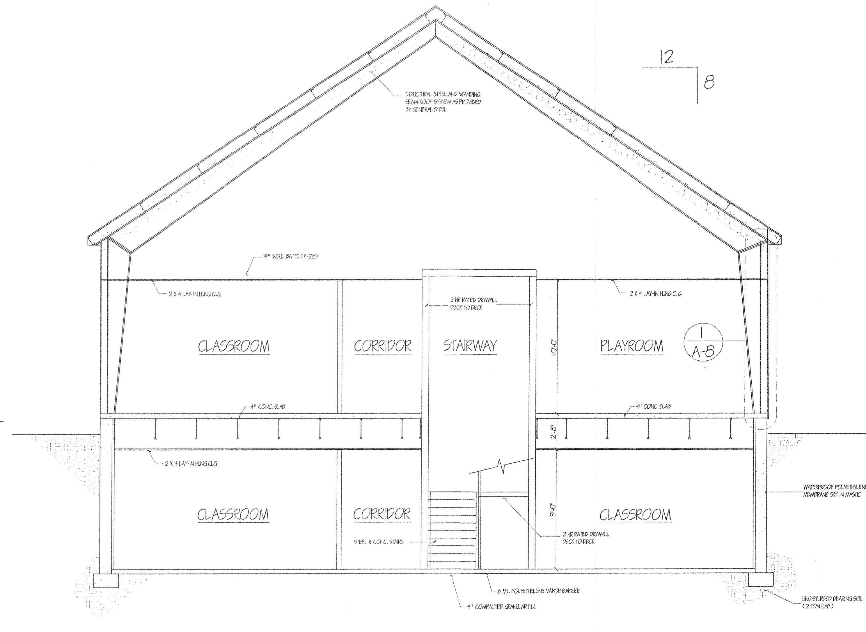
SECTION 2 A-7 1/4" = 1'-0"
