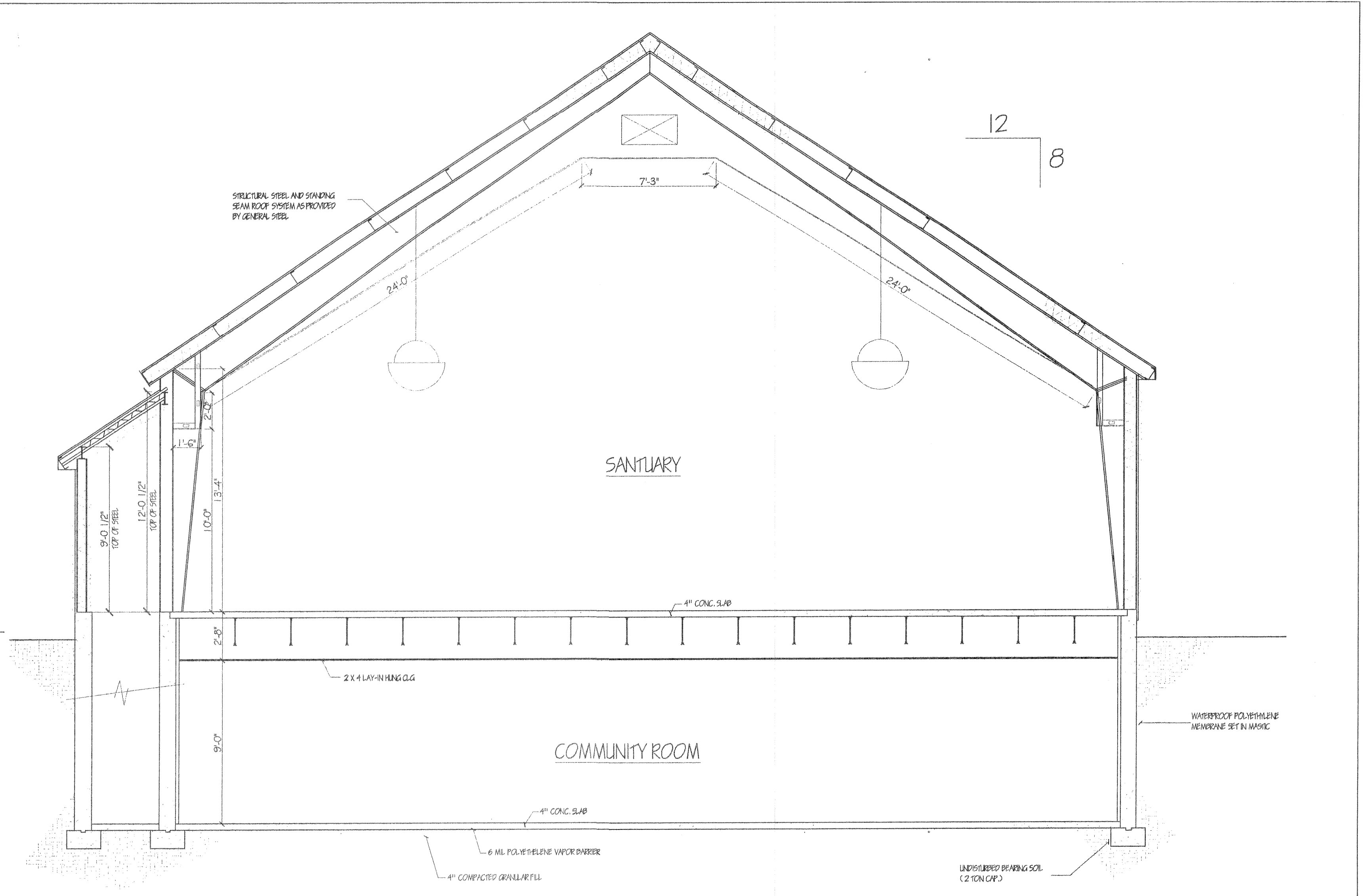
SECTION 2 A-6 1/4" = 1'-0"
