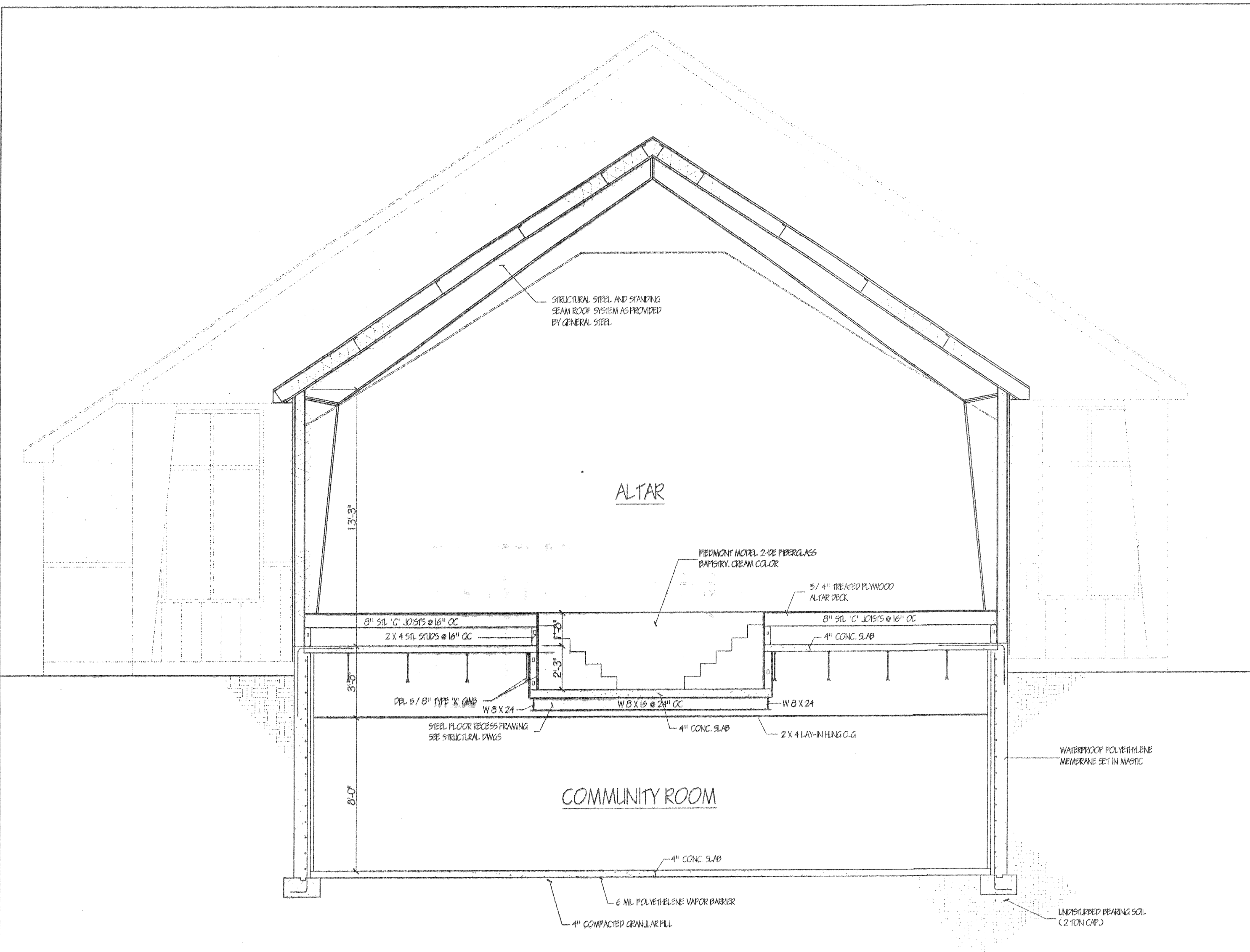
SECTION 1 A-6 1/4" = 1'-0"
